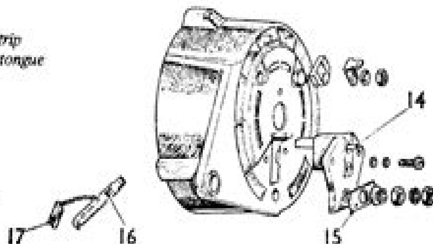
Exploded view of Lucas 11AC alternator
