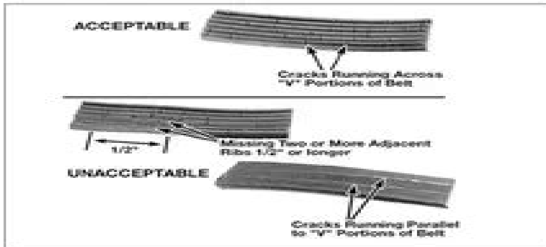
24.4 Small cracks in the underside of a V-ribbed belt are acceptable - lengthwise cracks, or missing pieces that cause the belt to make noise, are cause for replacement
