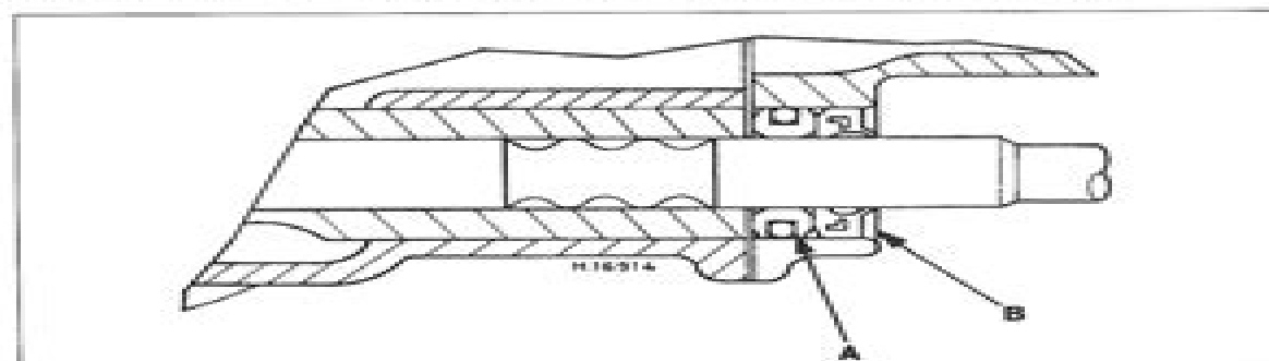
8.16 Selector shaft nylon bush and O-ring (A) fitted behind main oil seal (B)
