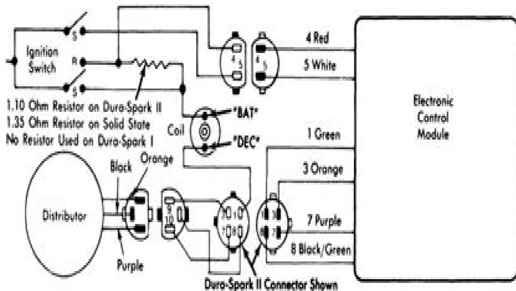
Fig. 2: 1976-79 Motorcraft Dura-Spark I & II Ignition System Wiring Diagram
