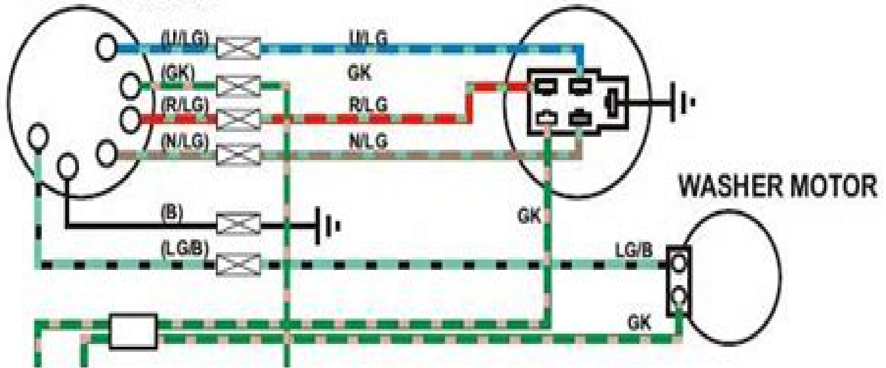
† WIPER/WASHER SWITCH
