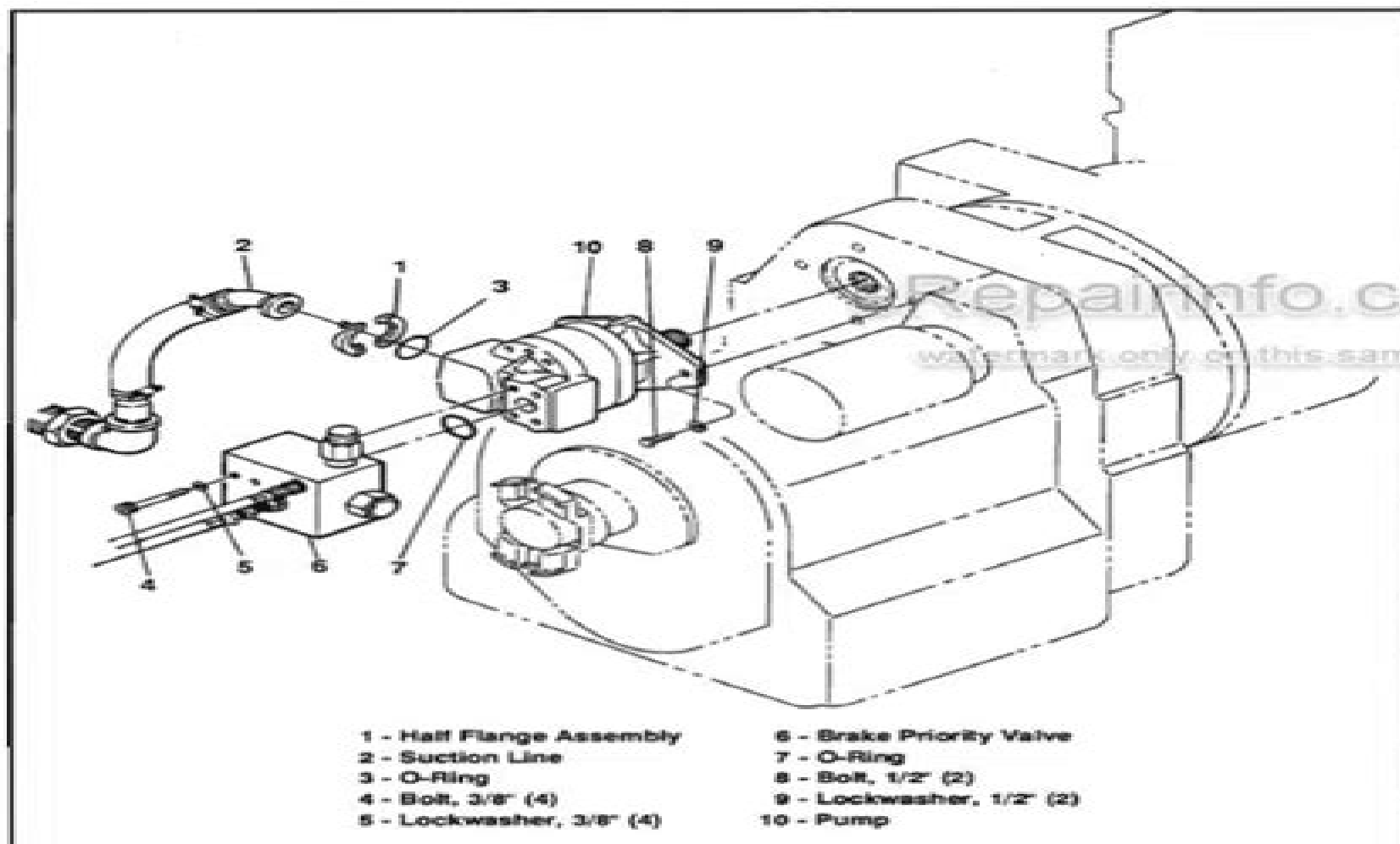
Figure 3-18 Hydraulic Pump Removal
