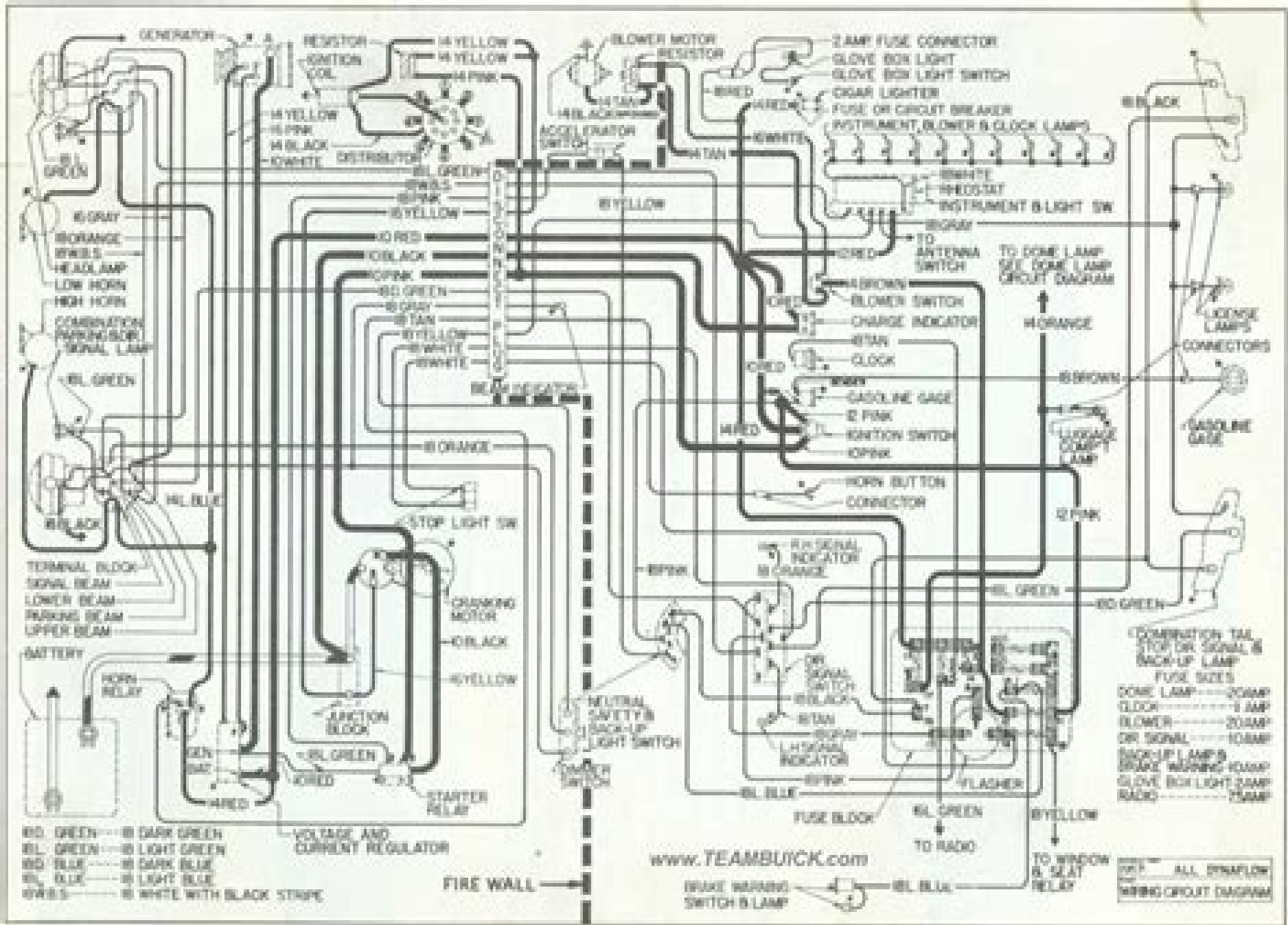
Figure 10-77—Chassis Wiring Diagram (Continued)
