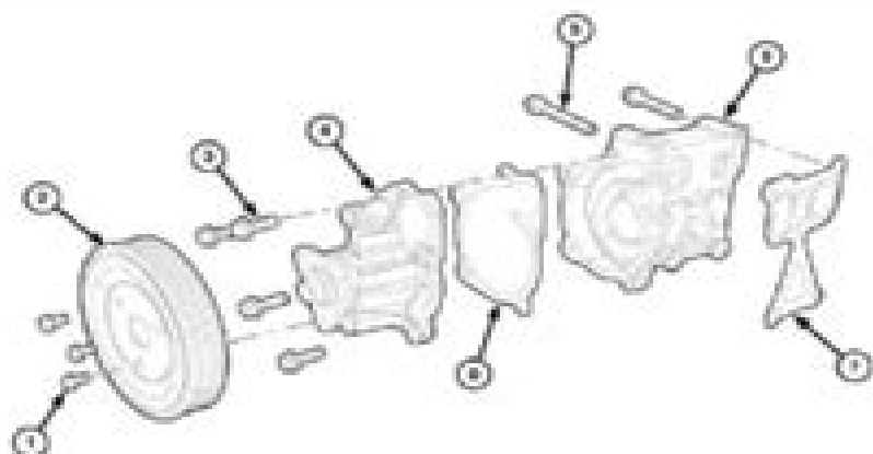
Fig. 1. Water pump pulley, adjuster and locknut
