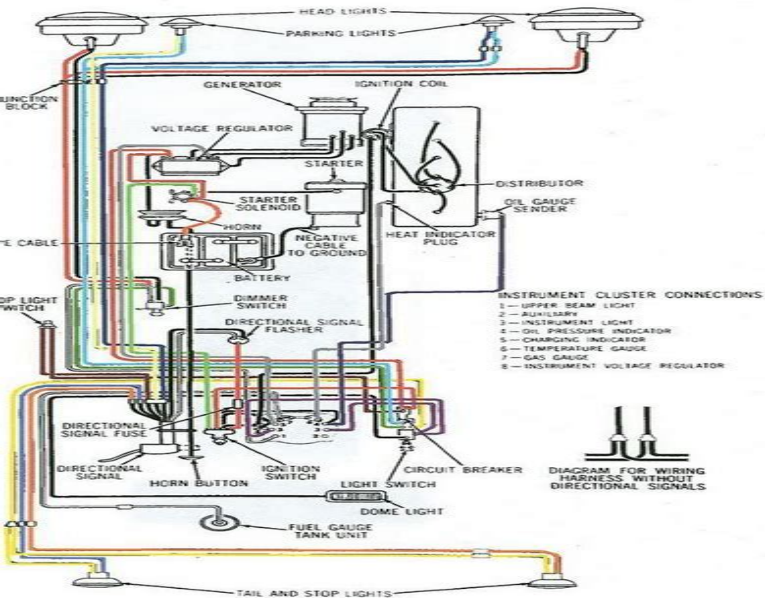
FIG. 18—WIRING DIAGRAM
