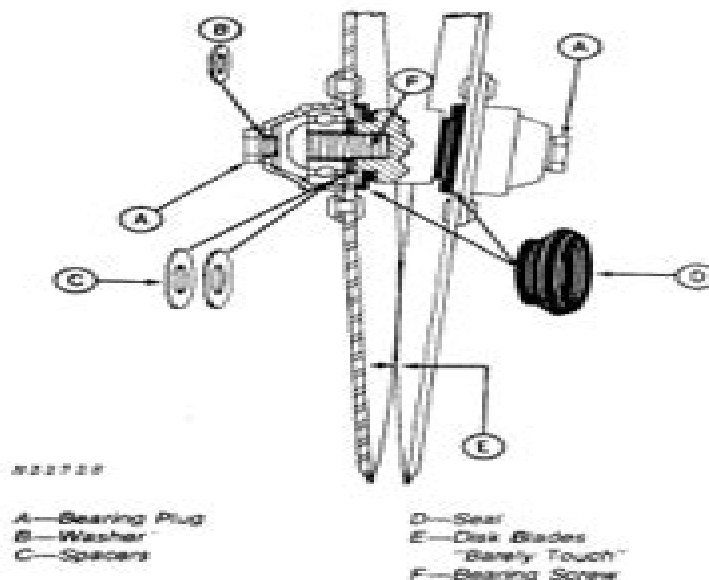
Fig. 104-Blades and Bearings
