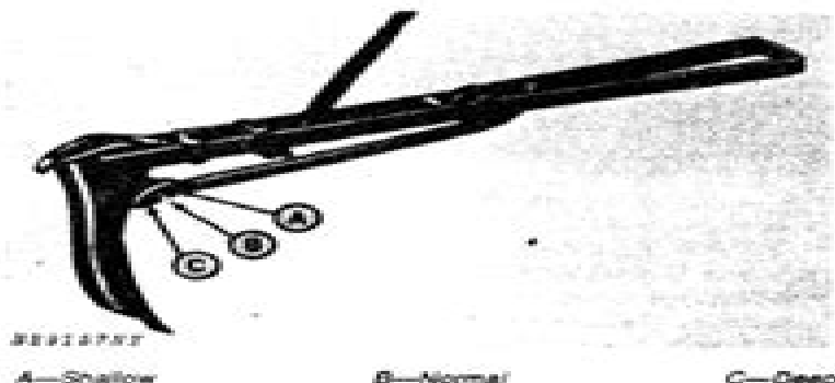
Fig. 103-Opener Adjustment
