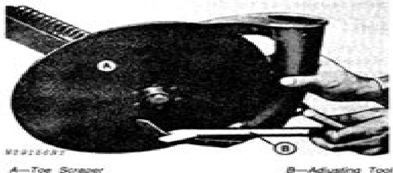
Fig. 102-Adjusting Toe Scraper
