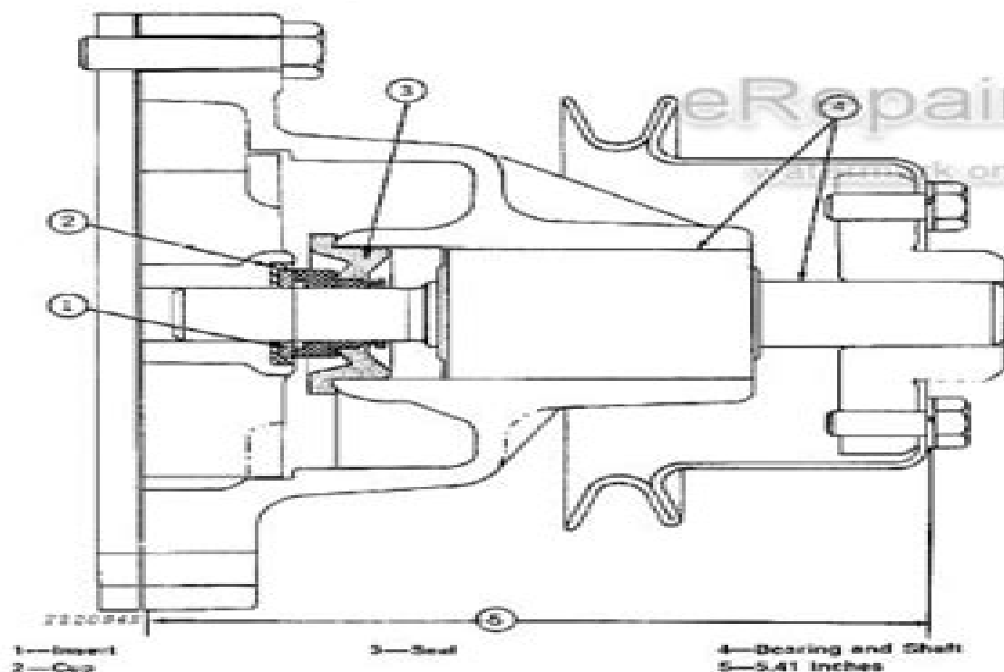
Fig. 2—Cutaway View of Water Pump Assembly
