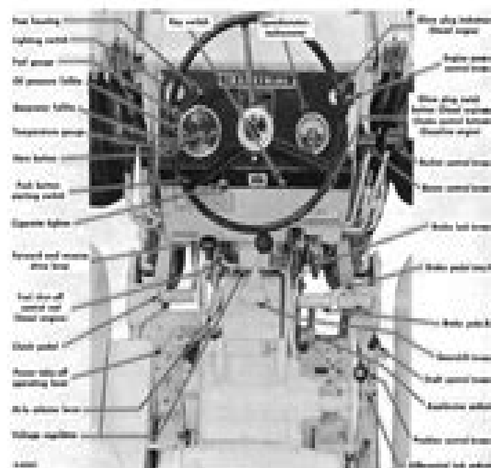
FIGURE 1 Instrument panel of a loader tractor.
