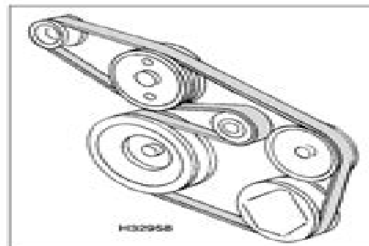
21.13b ... and on models with air conditioning – 2.0 and 2.2 litre engines
