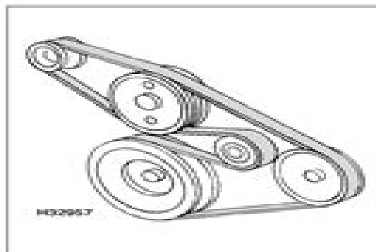
21.13a Auxiliary drivebelt configuration on models without air conditioning ...
