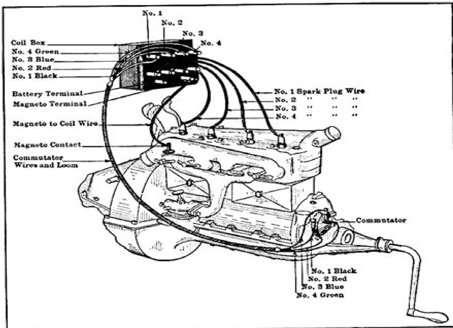
Fig. 16.—View of Ford Power Plant Showing Main Parts of the Ford Ignition System. Note Location of Timer and Induction Coil Box.
