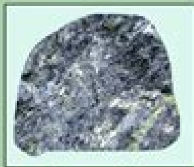
Blue schist
