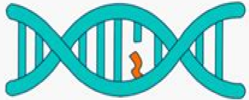
Mutated Gene
