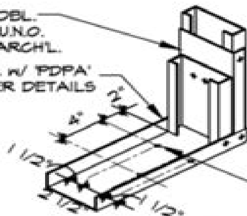
TYP. JAMB ASSEMBLY @ SLAB
