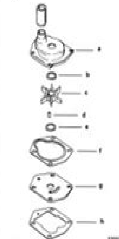
a - Cover b - Washer (above impeller) c - Impeller d - Key e - Washer (below impeller) f - Cover Gasket g - Base Plate h - Base Gasket
