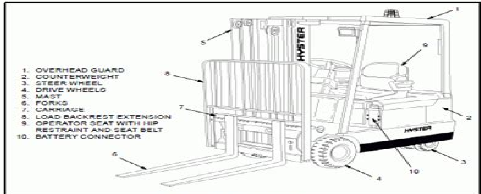
FIGURE 1 - PARTS OF THE TRUCK
