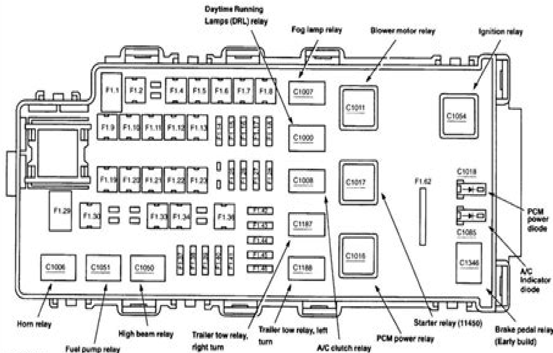
Fig 5: Identifying Battery Junction Box Components
