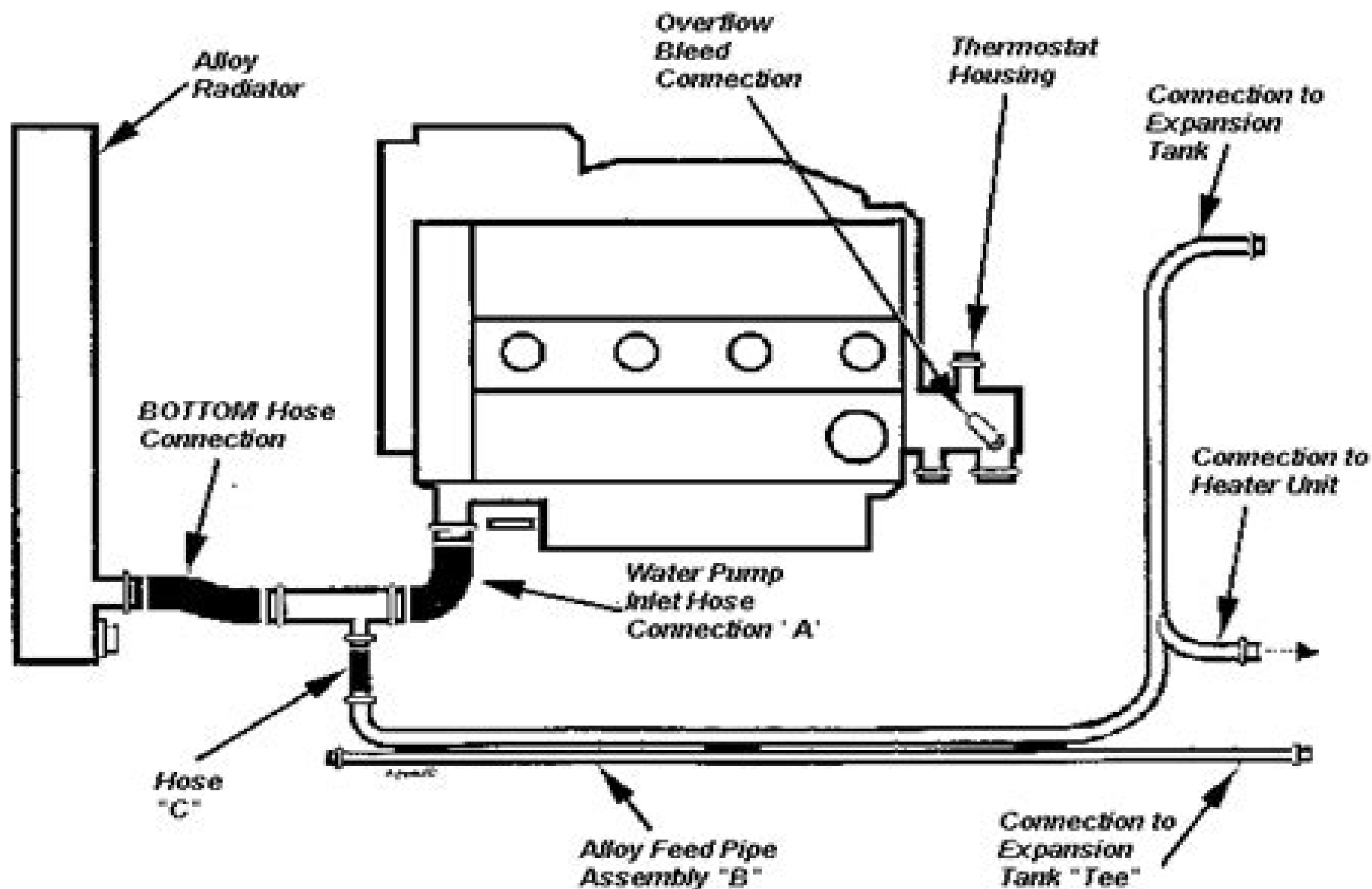
DIAGRAM 51 (Ducted Nose)
