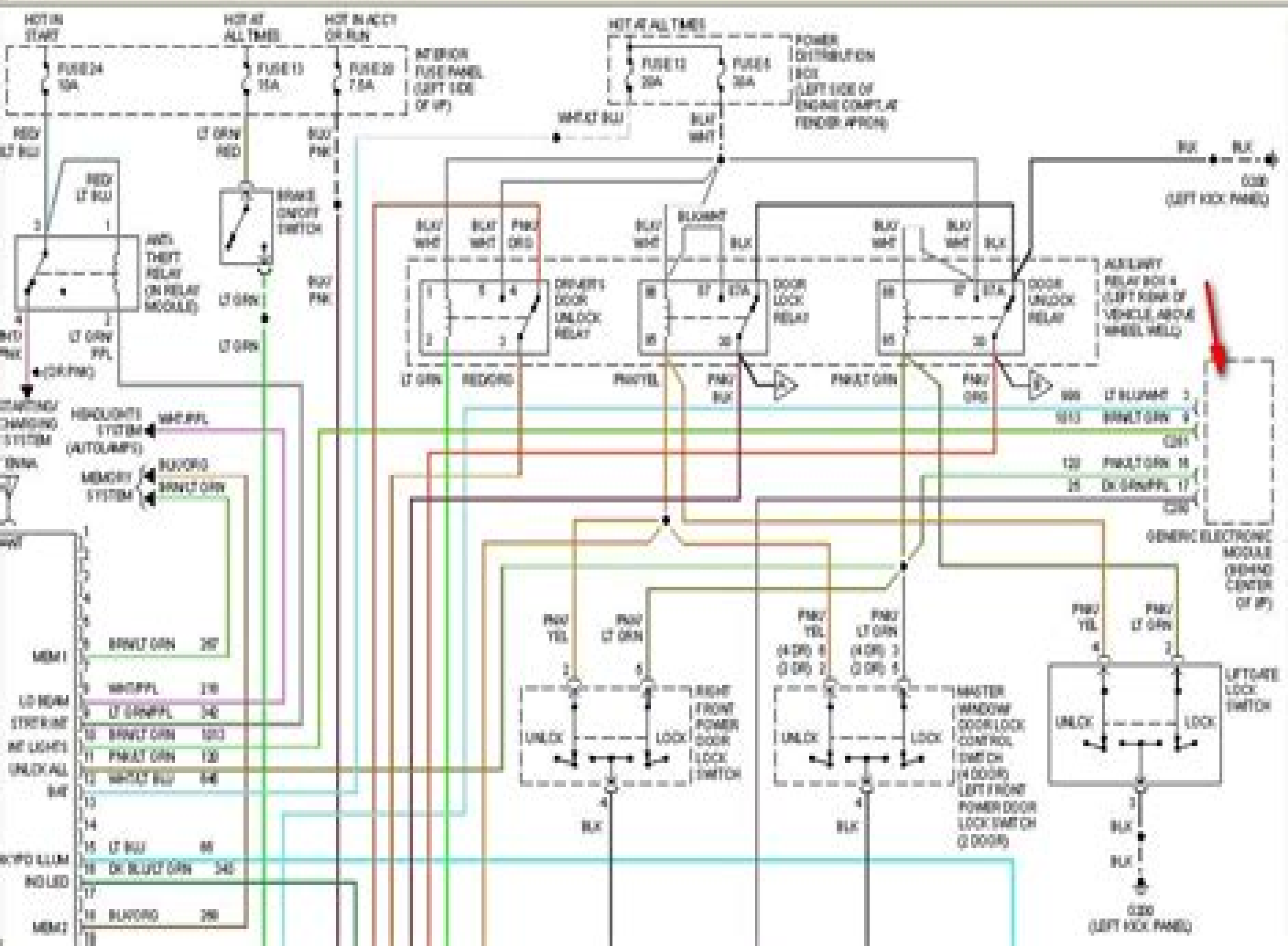
Fig. 1. Remote Keyless Entry System Wiring Diagram (Excerpt)
