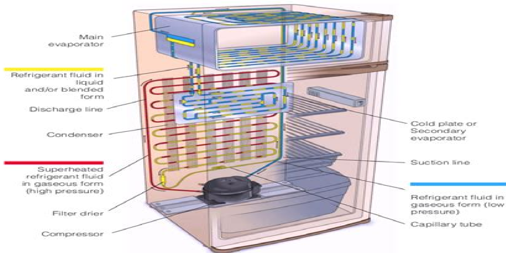
Figure 1 - Operation of a basic refrigeration system
