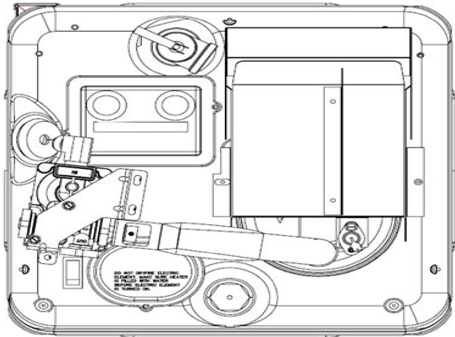
Typical Gas DSI/Electric Water Heater
