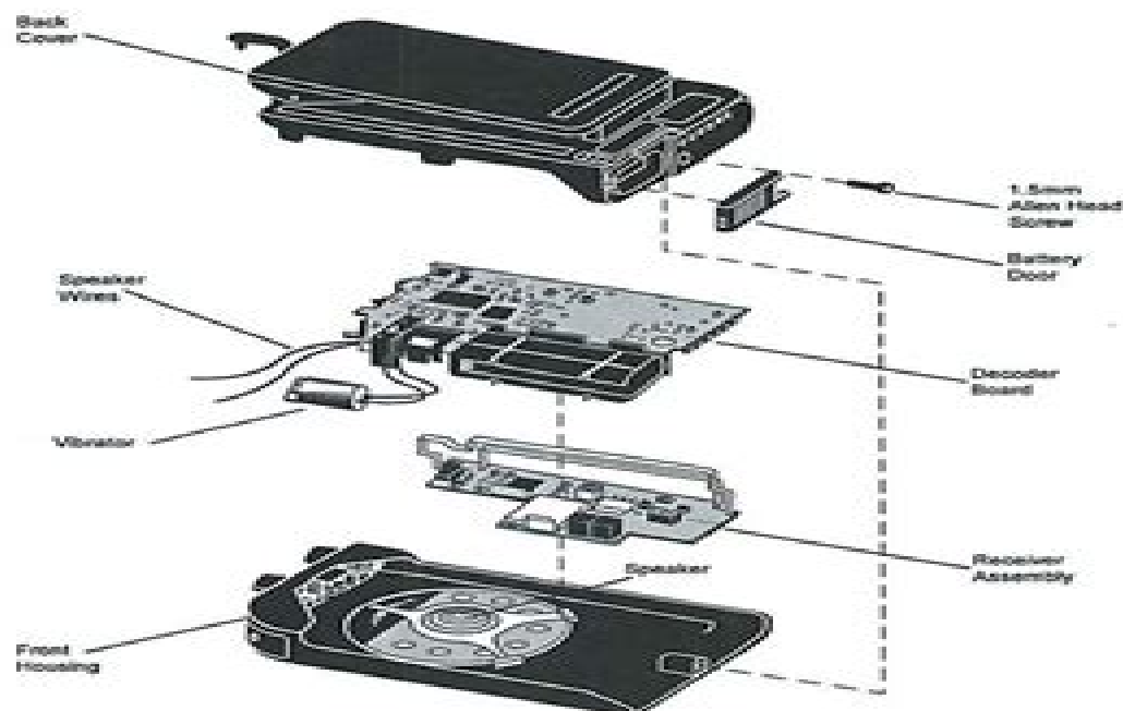
Figure 1. MINITOR IV - Major Components
