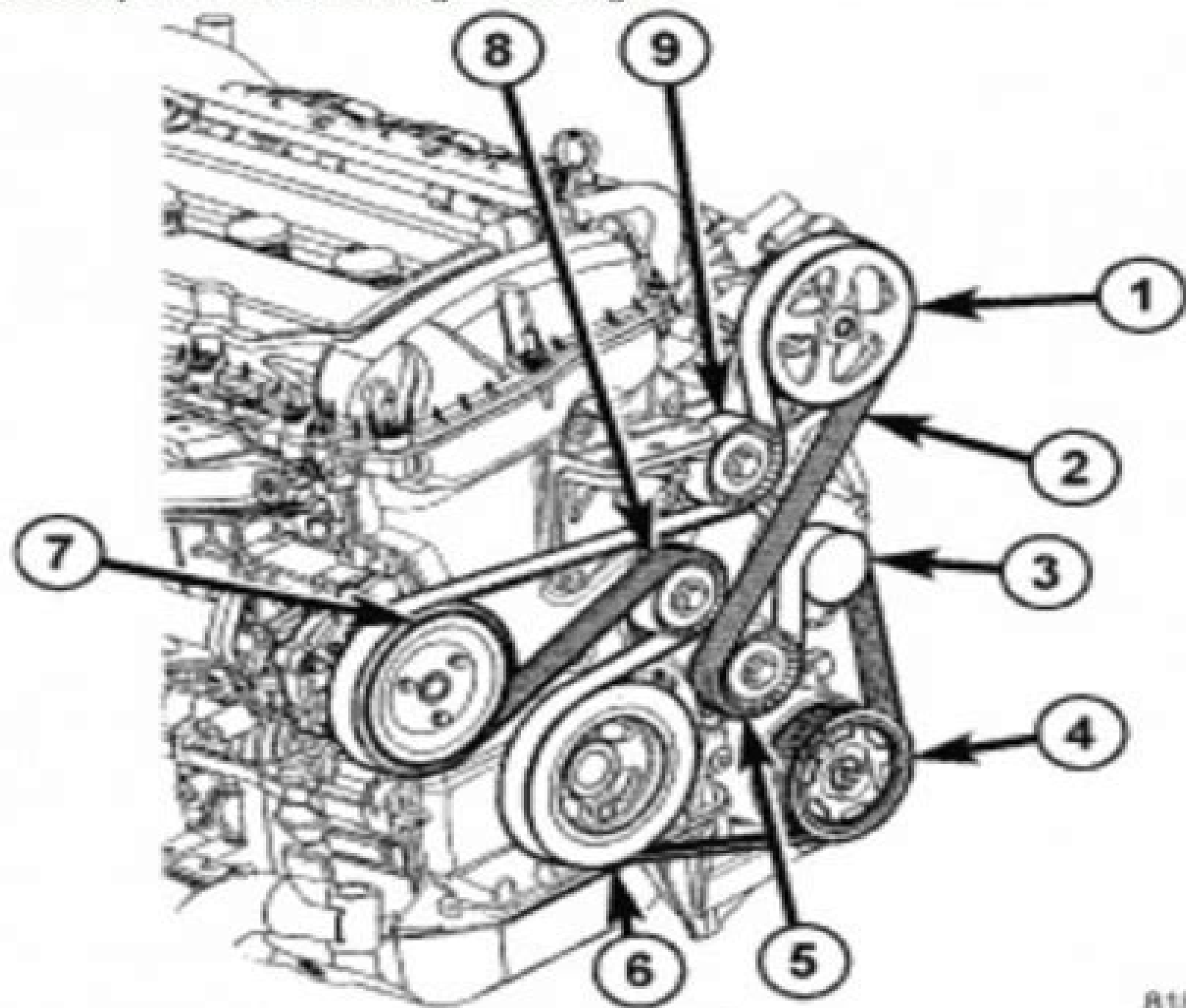
Fig 1: Accessory Drive Belt Routing - Gas Engine
