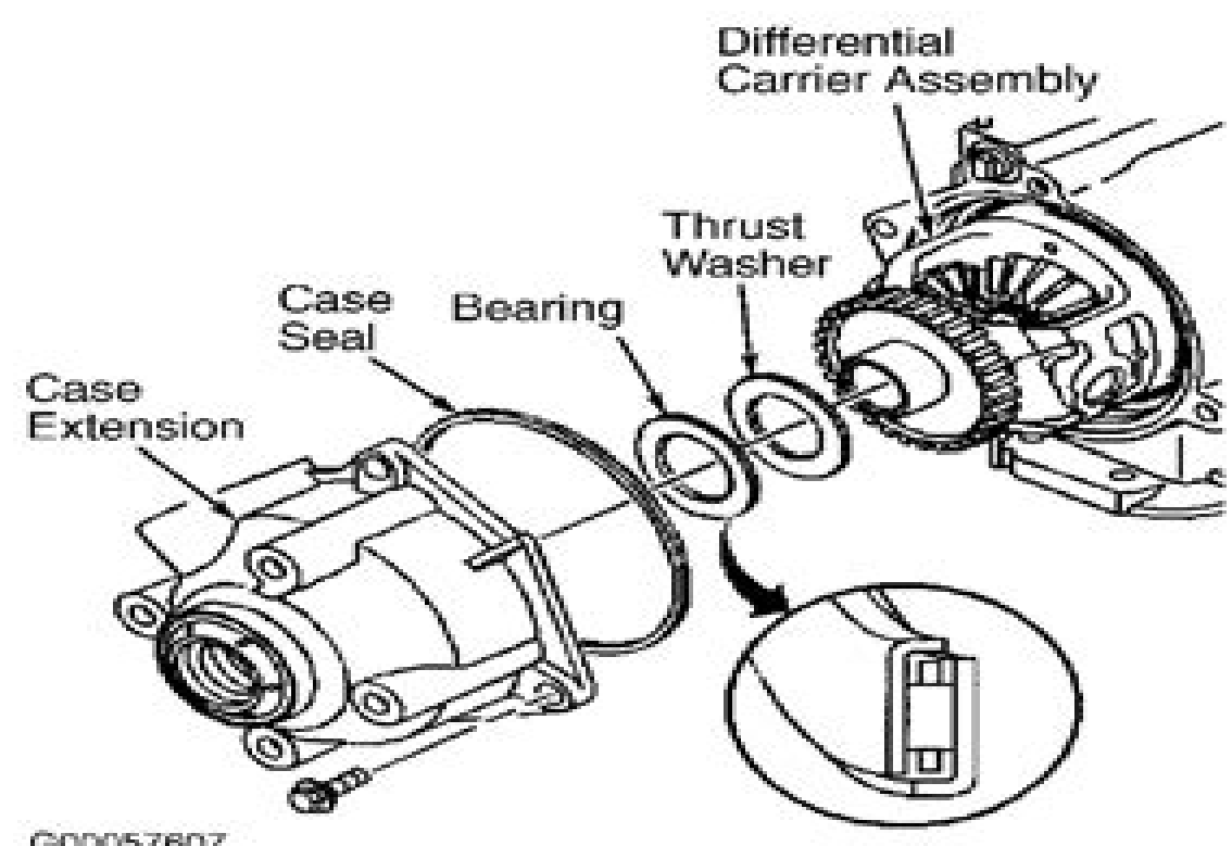
Fig. 19: Removing & Installing Case Extension Courtesy of GENERAL MOTORS CORP.
