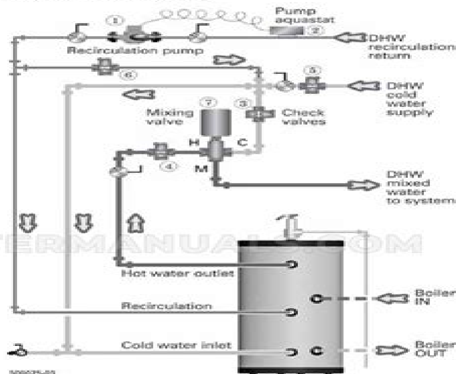
Figure 6 Recirculation piping
