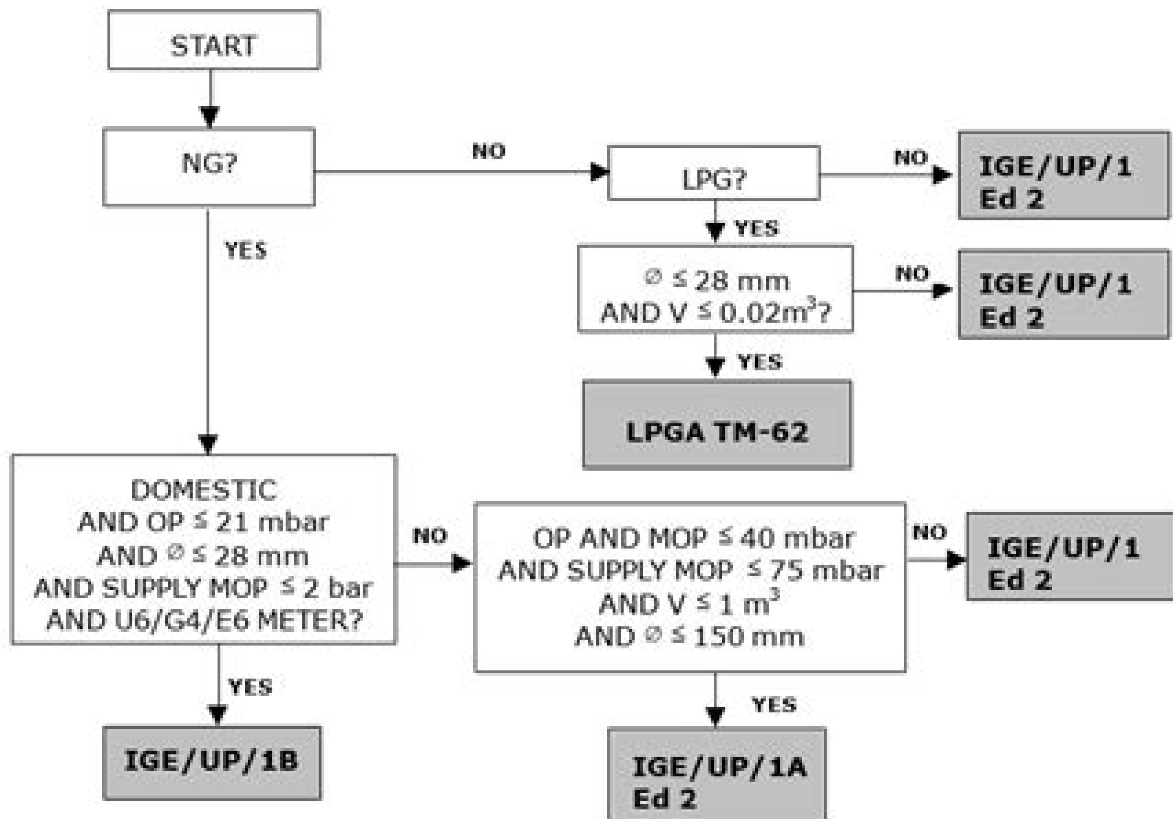
FIGURE 1 - RELATIVE PRESSURE LEVELS
