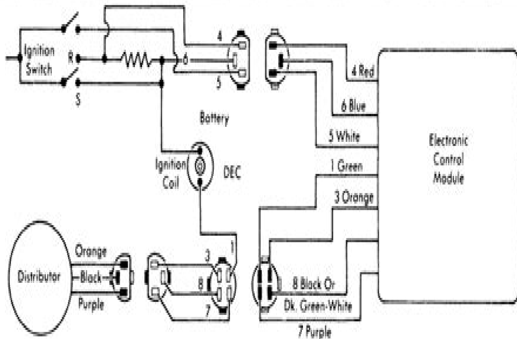
Fig. 1: 1975 Motorcraft Solid State Ignition System Wiring Diagram
