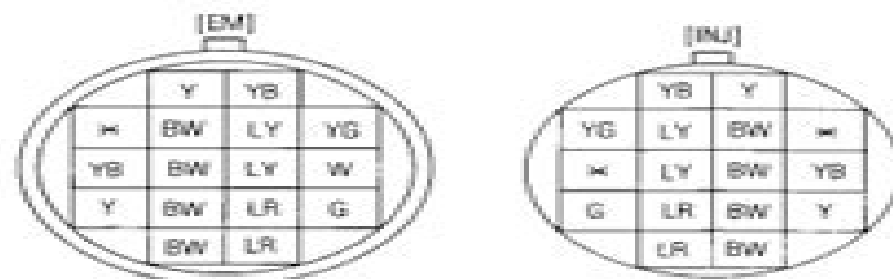
B-19 Connector Between Emission [EM] And Injector [INJ] Harness
