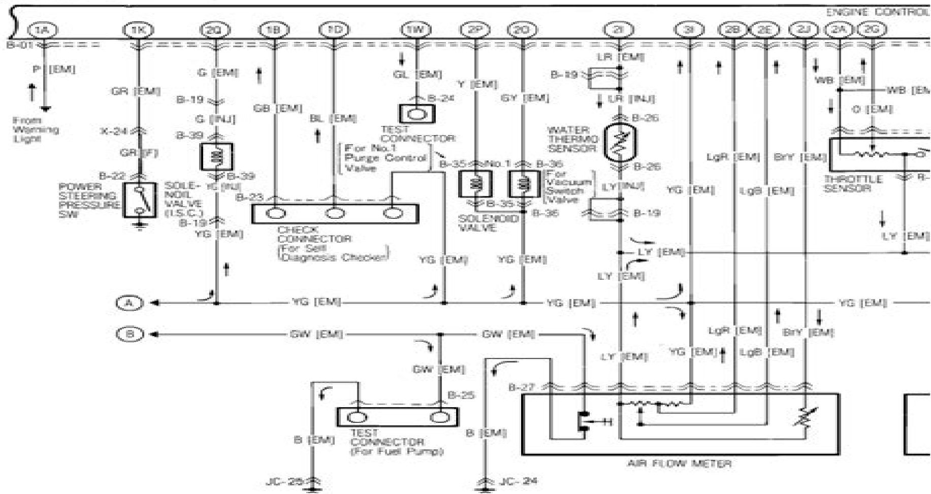
B-01 Engine Control Unit [EM]
