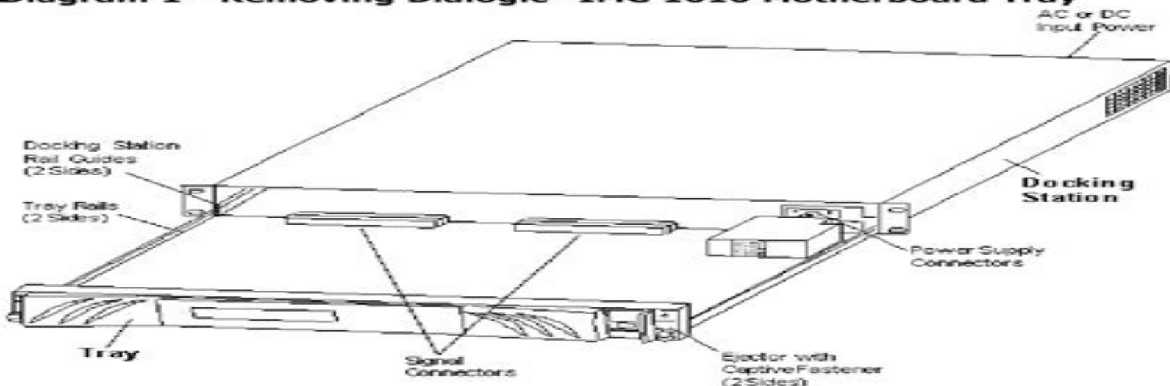
Diagram 1 - Removing Dialogic® IMG 1010 Motherboard Tray
