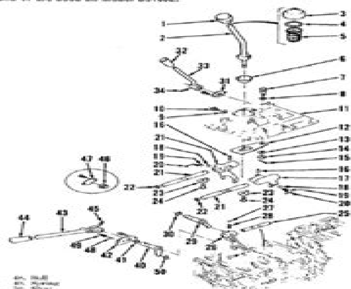
Fig. 79—Exploded view of shifter mechanism used on Models BS3000 and BS1000. Components 39 through 44 are used on Model BS1000 and components 45 and 47 are used on Model BS1000.
