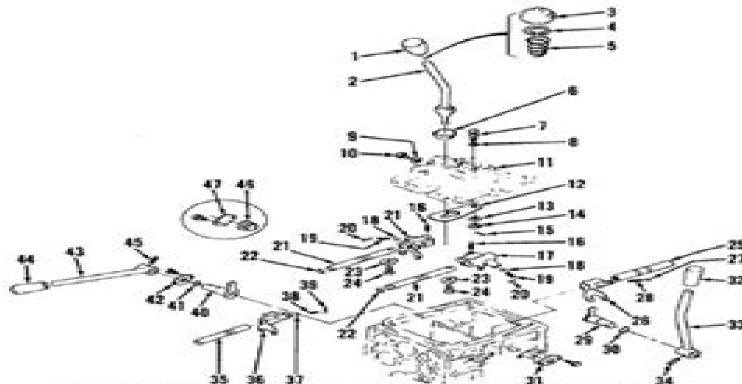
Fig. 79—Exploded view of shifter mechanism used on Models BS3000 and BS1000. Components 39 through 44 are used on Model BS1000 and components 45 and 47 are used on Model BS1000.
