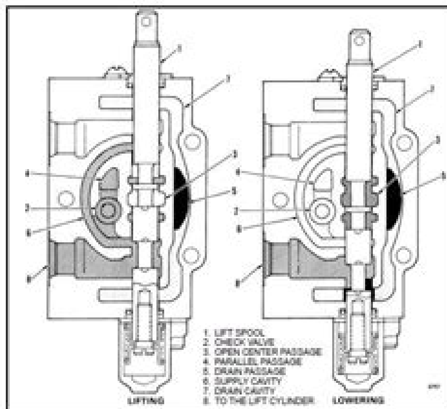
FIGURE 3. LIFTING AND LOWERING
