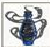
Voidberry Potion
