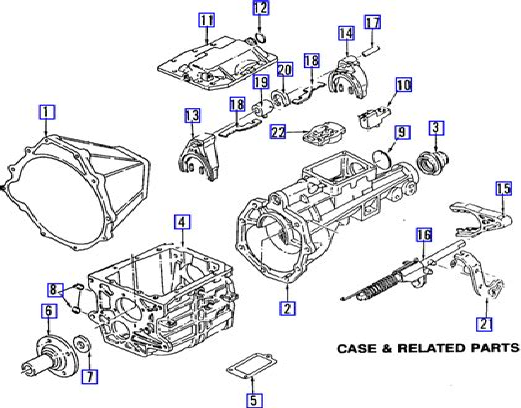
MANUAL TRANSMISSION 2WD, 3.1 LITER
