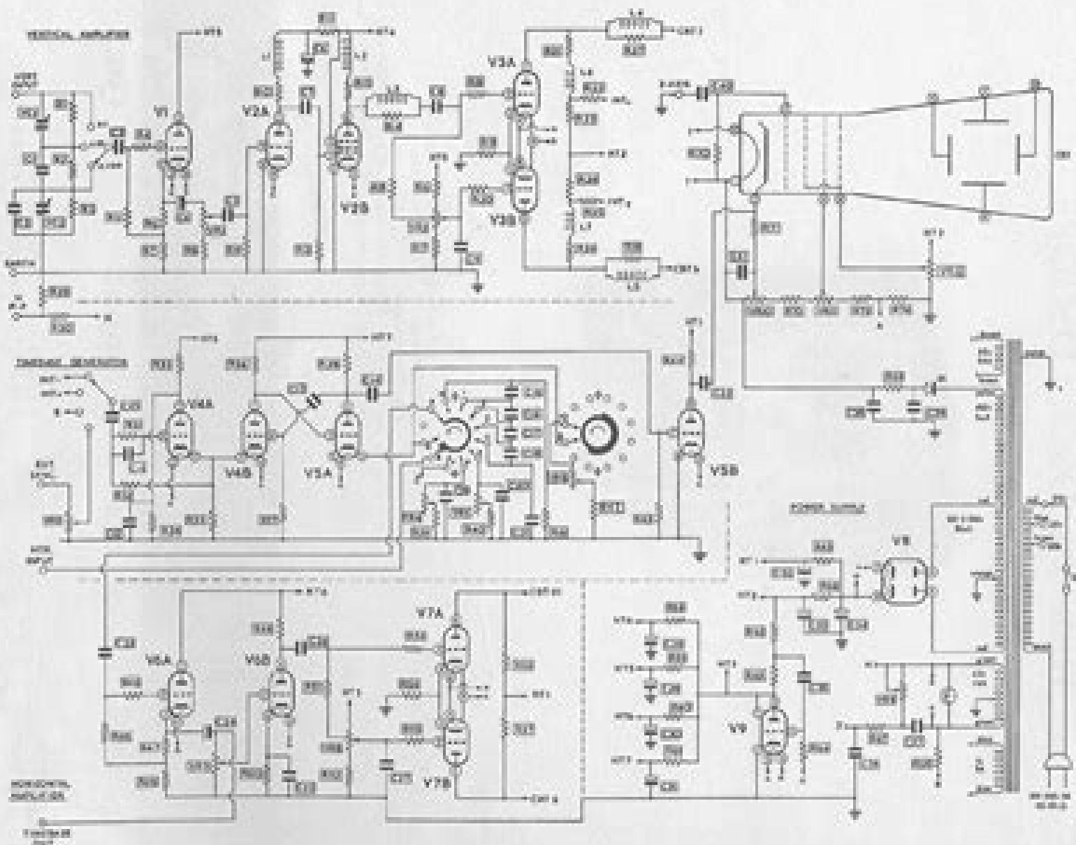
CIRCUIT DIAGRAM OF THE HEATHKIT LABORATORY and GENERAL PURPOSE OSCILLOSCOPE Model 10-12U
