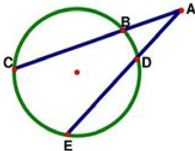
Two Secants
