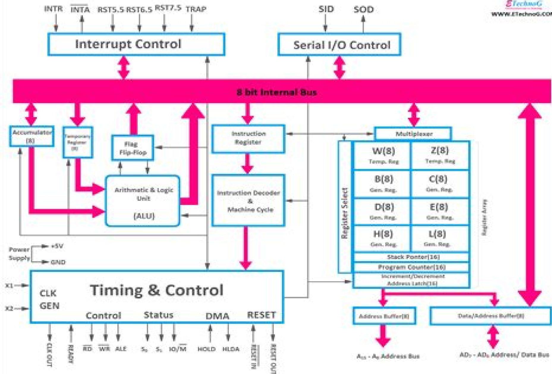
Microprocessor 8085 Block Diagram and Architecture
