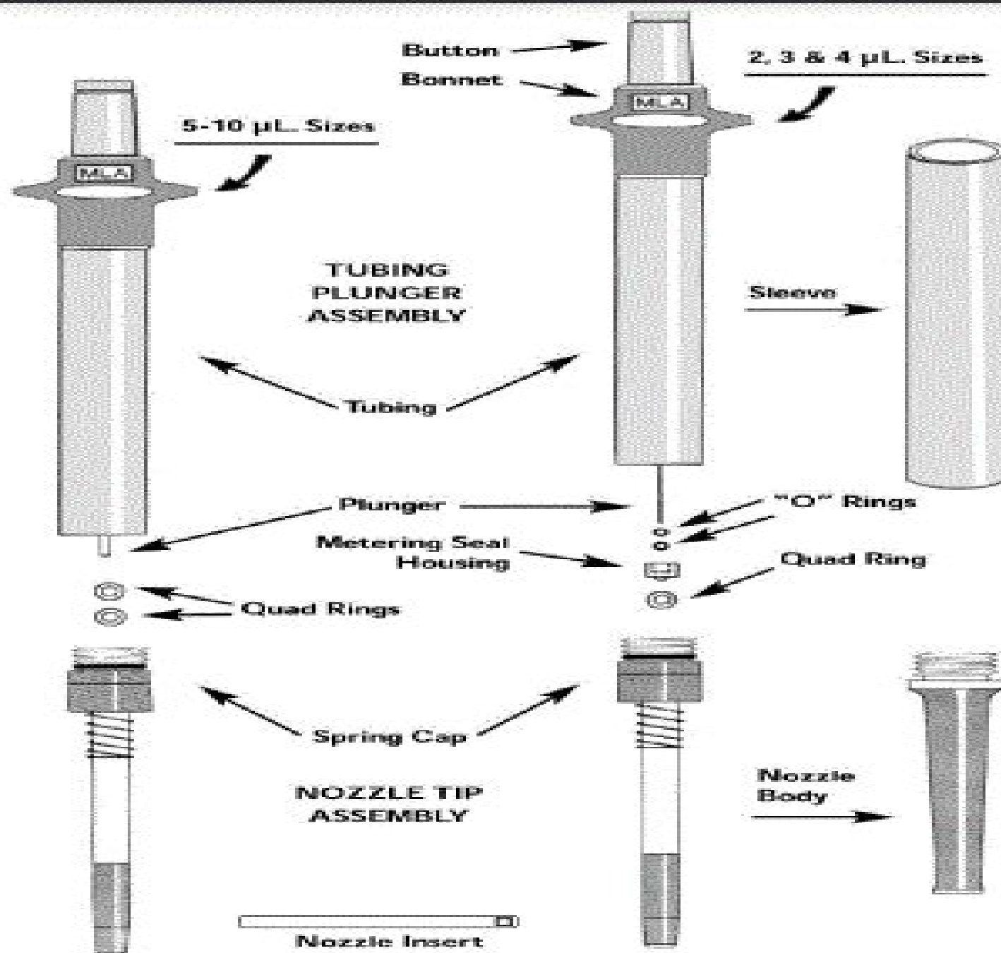
Figure 3 : Pipette Disassembly and Seal Replacement
