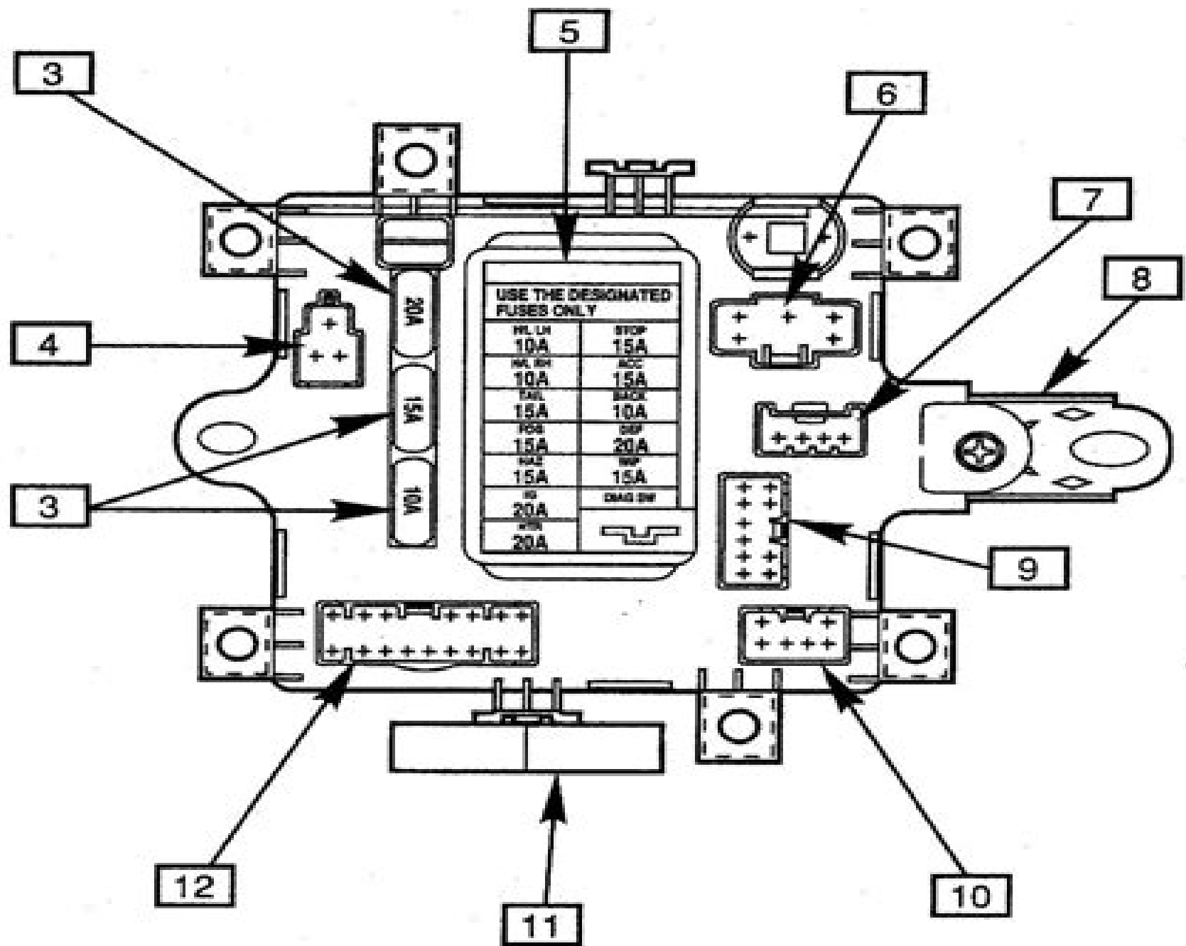
Junction Block, Bottom View
