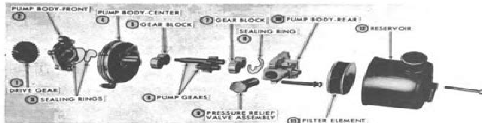
Figure 18 Power Assisted Steering Pump Components
