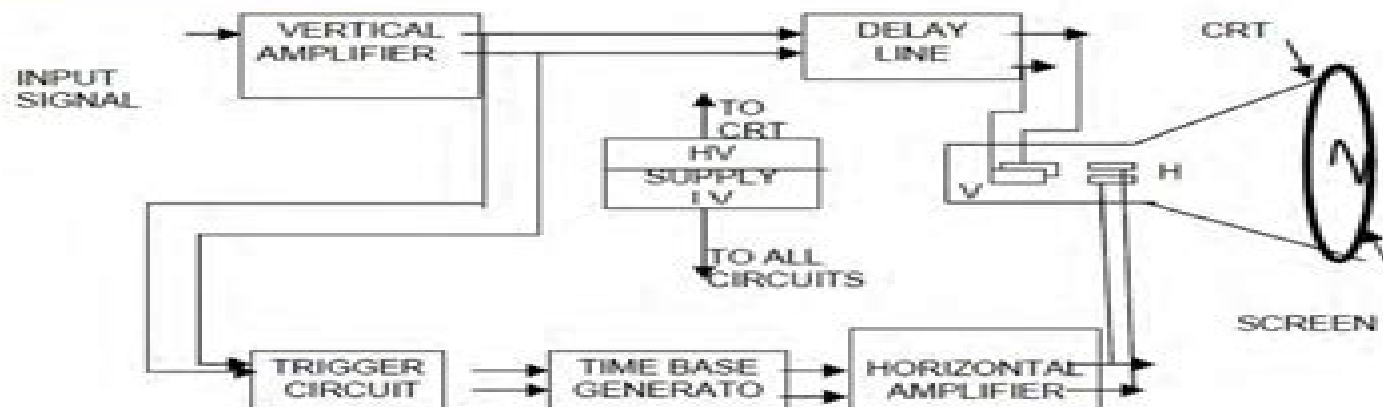
Figure A: BLOCK DIAGRAM OF CRO
