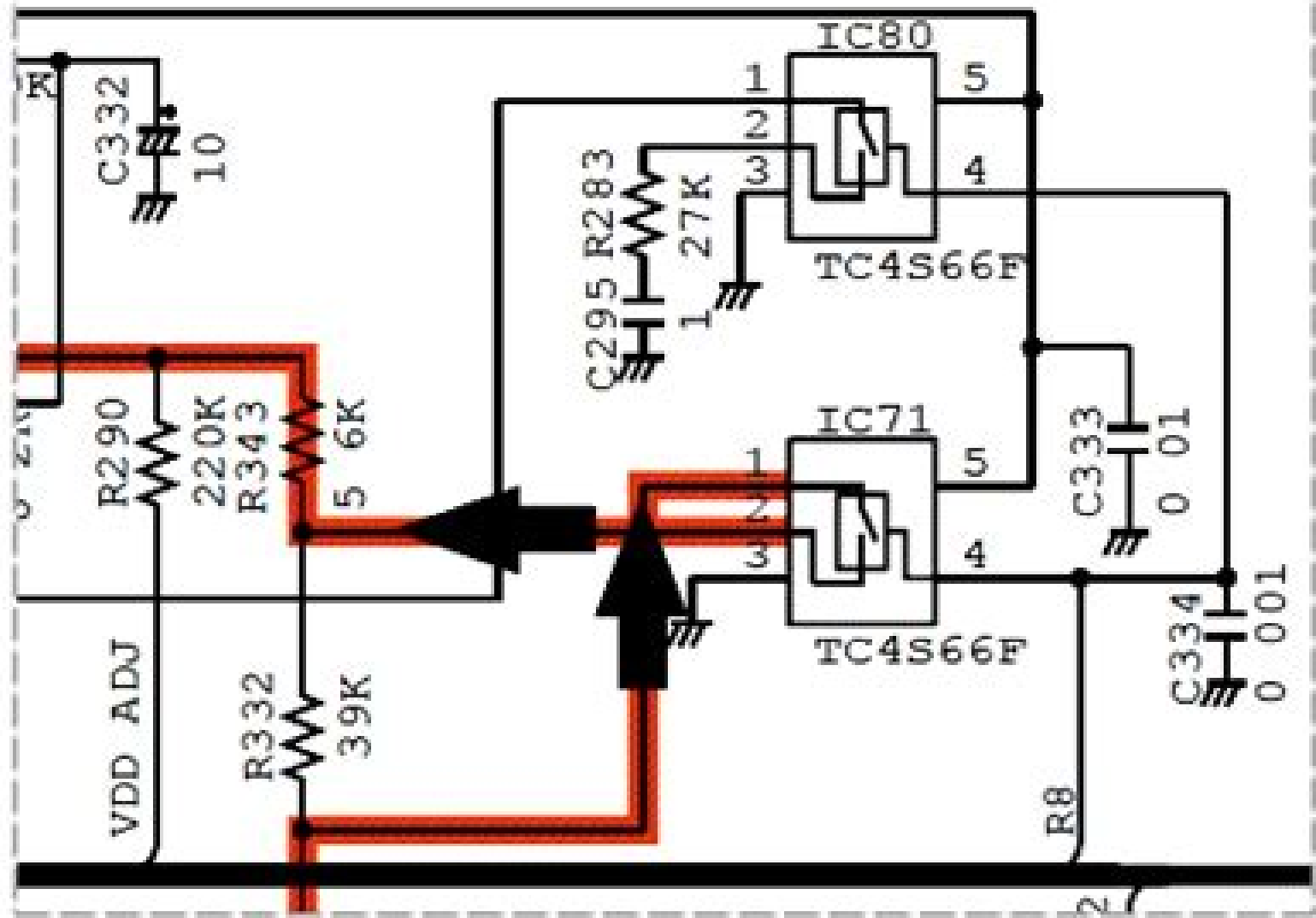
Preview: ICOM IC-A210 schematic diagram
