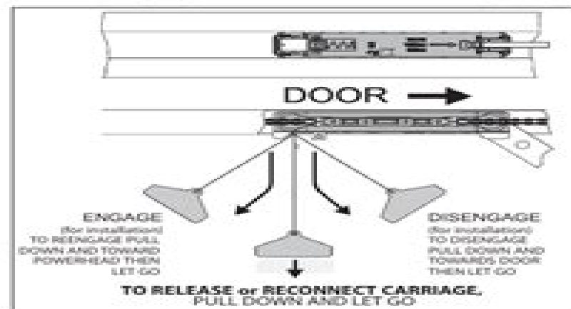
FIG. 6-4 Carriage Release (cut away view) 12/2010
