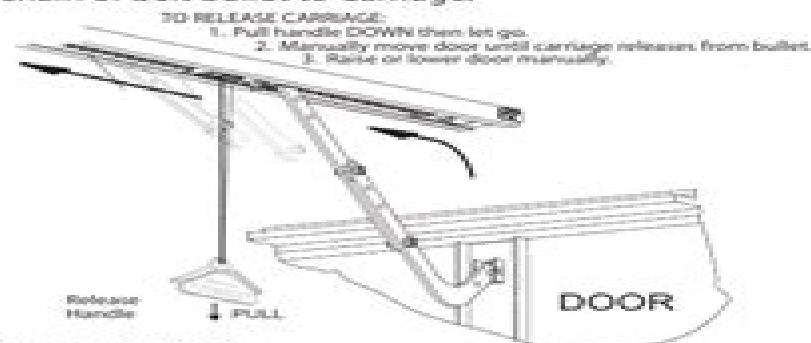
FIG. 6-3 Carriage Release
