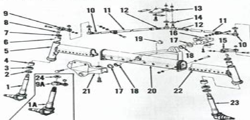
Fig. 1—Exploded view of row crop type wide adjustable front axle. All purpose type front axle is similar except that center member (20) is reversed to provide shorter wheelbase. Note that later models are equipped with spindles (1A) and steering arms are retained by a nut as shown in inset. All parts except center steering arm (13) and inner tie-rod ends (12) are interchangeable between row crop and all purpose types. Refer to Figs. 2 and 3 for center steering arm views.
