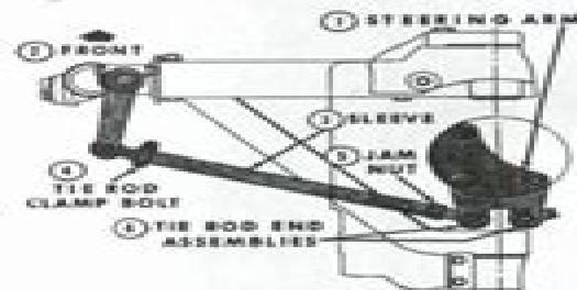
Fig. 2—When checking toe-in on row crop wide adjustable axle, be sure steering arm is centered as shown. View is from top. When installing center steering arm, be sure steering motor is centered and install arm as shown.
