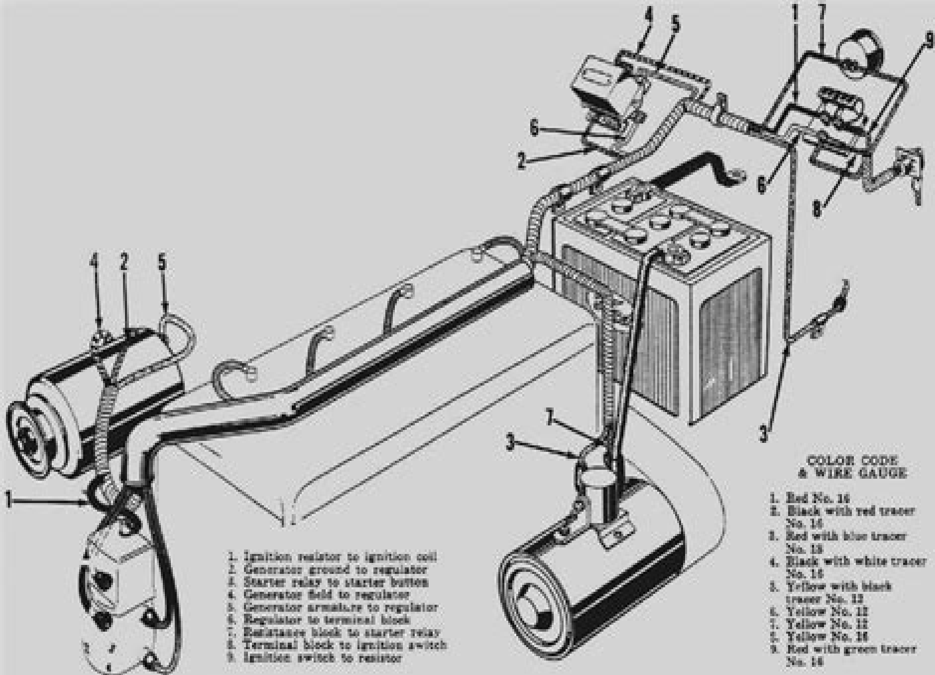
Fig. 1043—Electrical system on model 8N prior to tractor serial 263884.
