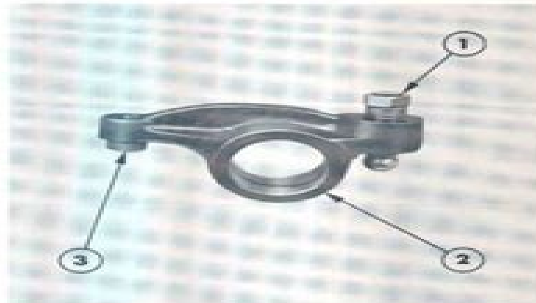
Figure 8 Intake Valve Rocker Arm Assembly
