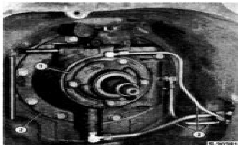
Figure 78 Transmission Pump and Oil Distributor Removal
