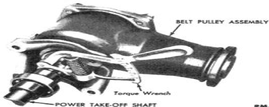
Fig. 53—Checking Driven and Drive Gear Torque
