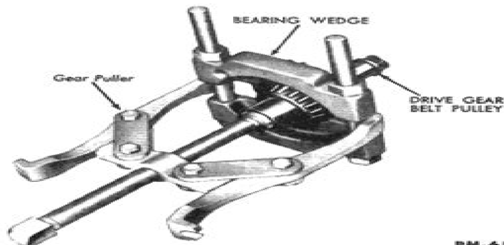
Fig. 52—Removing Bearing from Drive Gear
